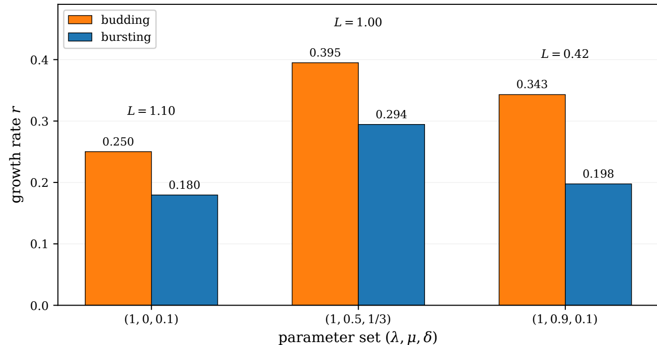
Matched R_0 = 2 and mean productive lifetime ( c = 1 )
